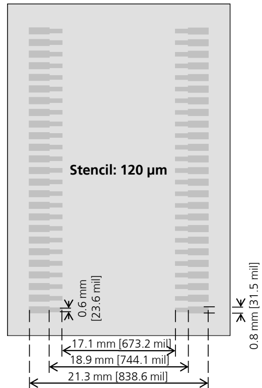
Figure 48: LEON-G100/G200 paste mask
