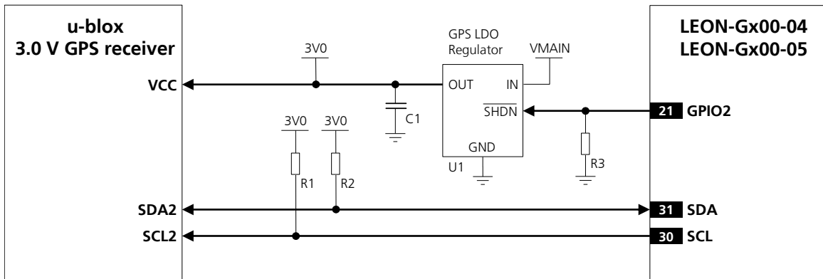
Figure 35: Application circuit for LEON-Gx00-04 and LEON-Gx00-05 versions and u-blox 3.0 V GPS receivers
