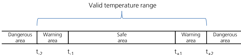
Figure 58: Temperature range and limits
