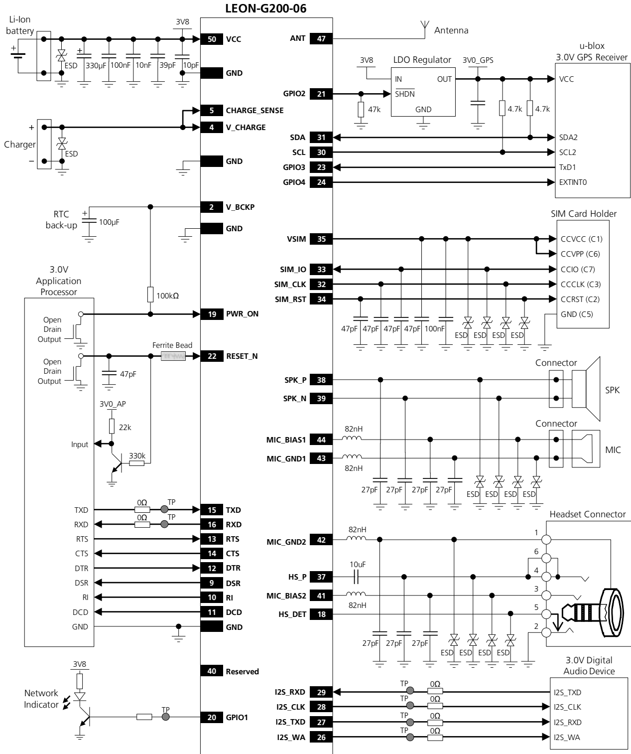
Figure 44: Example of schematic diagram to integrate LEON-G200-06 module in an application board, using all the interfaces
