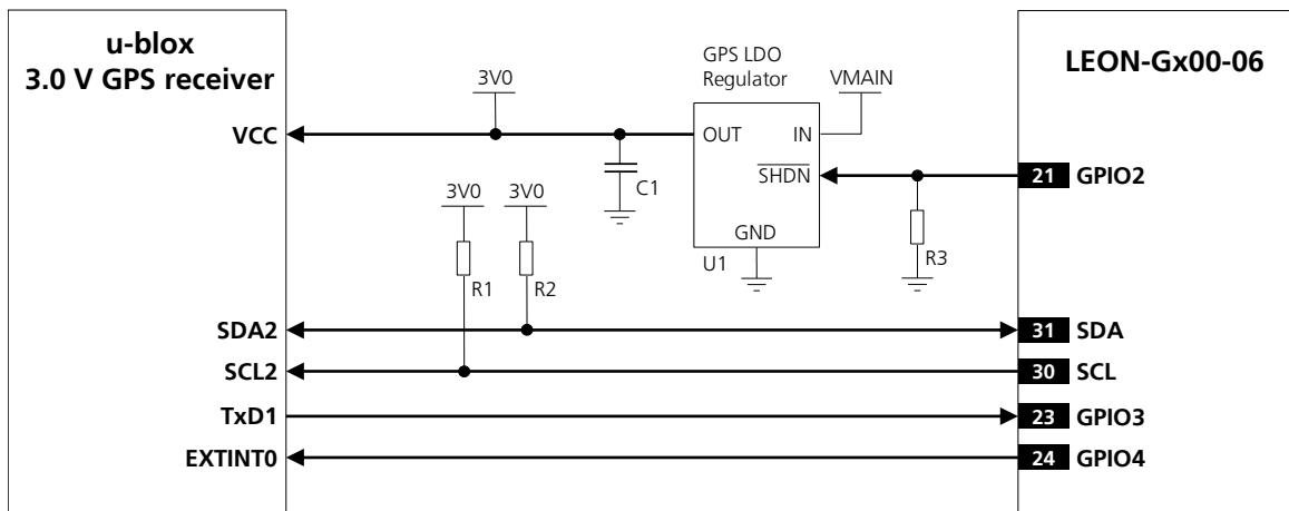
Figure 34: Application circuit for LEON-Gx00-06 versions and u-blox 3.0 V GPS receivers
