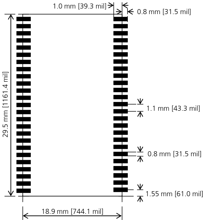
Figure 47: LEON-G100/G200 footprint
