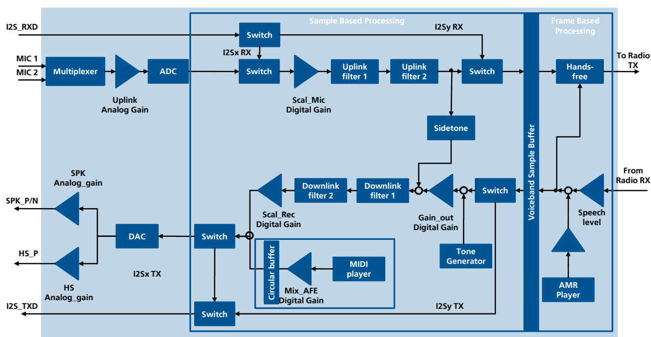
Figure 41: LEON-G100/G200 voice-band processing system block diagram
