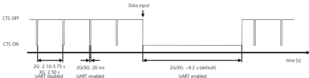
Figure 24: CTS behavior with power saving enabled (AT+UPS V =1) and HW flow control enabled: the CTS output line indicates when the UART interface of the module is enabled (CTS = ON = low level) or disabled (CTS = OFF = high level)
