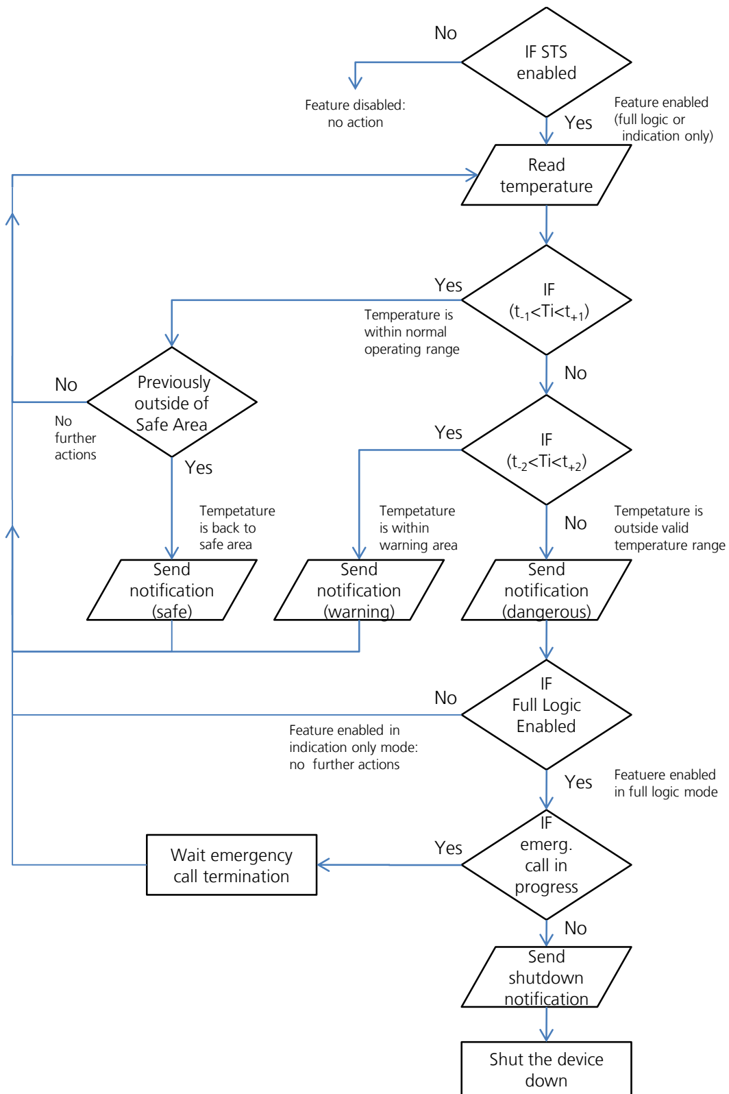
Figure 62: Smart Temperature Supervisor (STS) flow diagram
