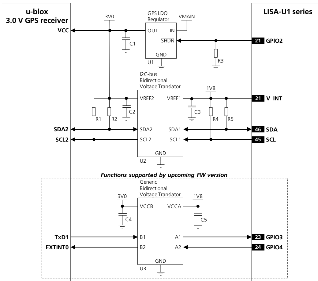
Figure 37: DDC Application circuit for u-blox 3.0 V GPS receiver
