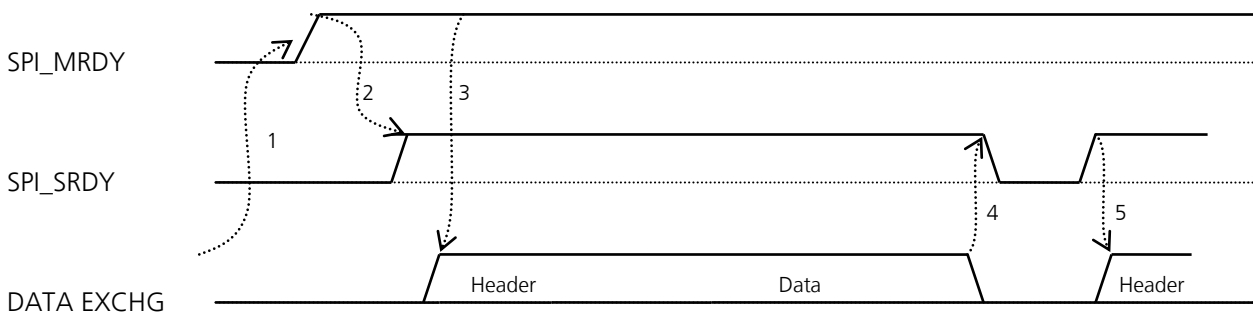
Figure 33: Data transfer initiated by application processor (master) with a sleeping LISA-U1 series module (slave)
