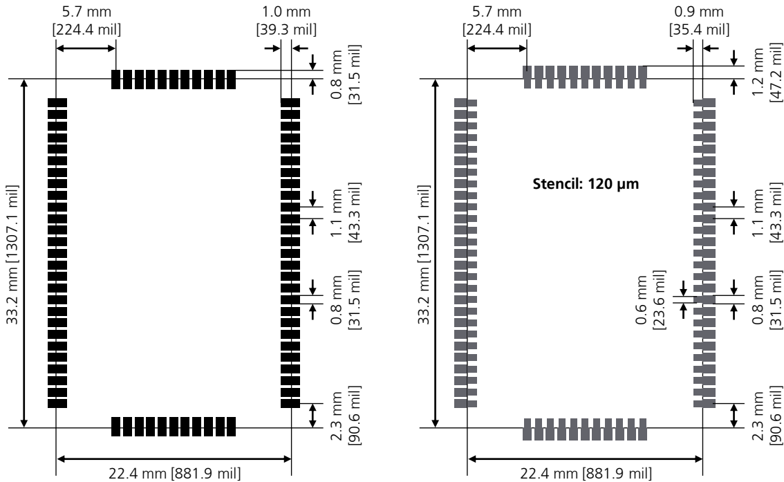
Figure 52: LISA-U1 series modules suggested footprint and paste mask
