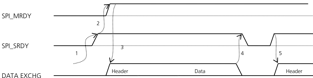
Figure 32: Data transfer initiated by LISA-U1 series module (slave), with a sleeping application processor (master)
