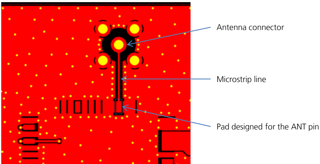
Figure 48: Layer 1 (top layer) of u-blox approved interface board for LISA-U1 series modules
