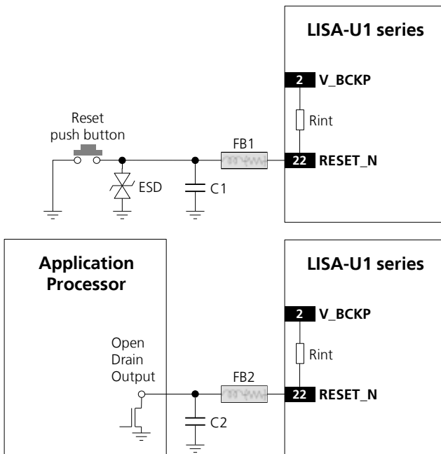
Figure 59: RESET_N application circuits for ESD immunity test
