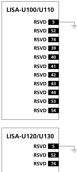
Figure 44: Application circuit for the reserved pins (RSVD)
