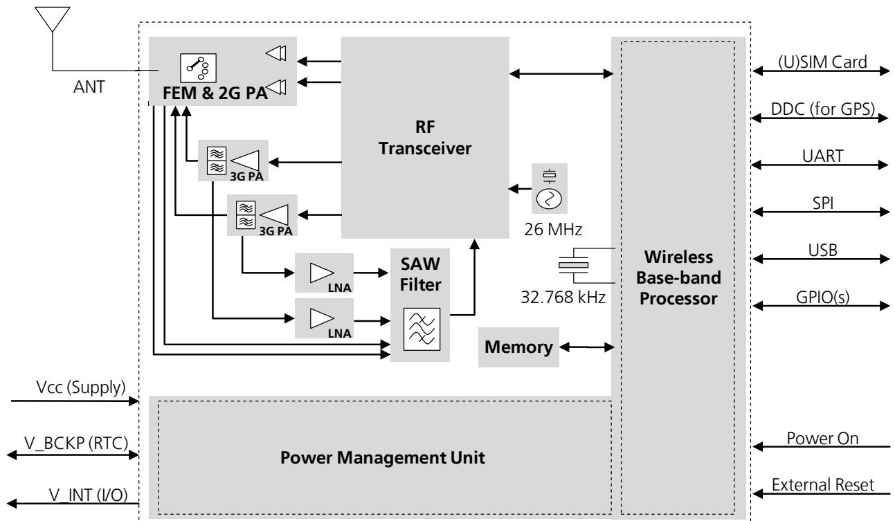
Figure 1: LISA-U100, LISA-U110 block diagram
