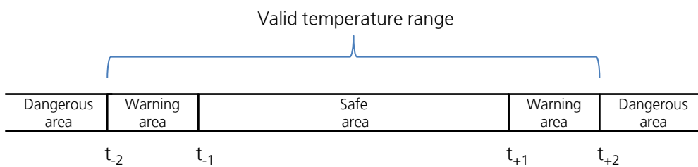
Figure 61: Temperature range and limits
