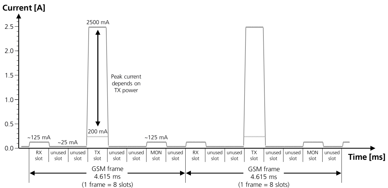
Figure 10: VCC current consumption profile versus time during a GSM call (1 TX slot, 1 RX slot), with VCC=3.8 V
