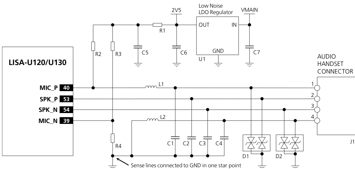
Figure 39: Handset mode application circuit
