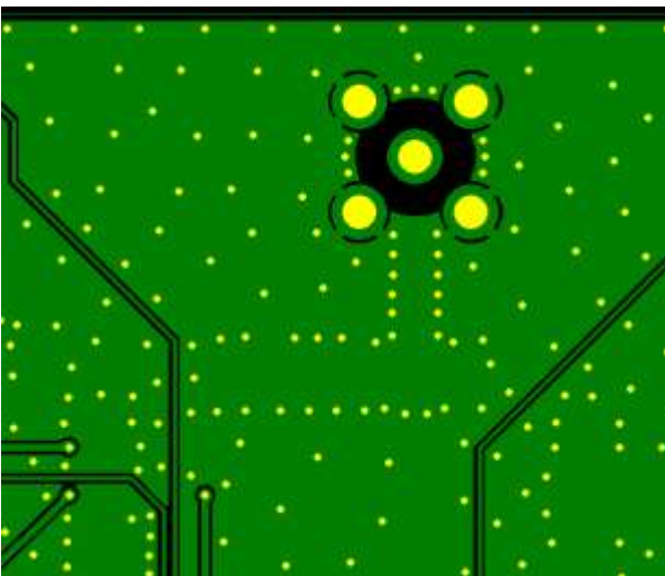
Figure 50: Layer 3 (inner layer) of u-blox approved interface board for LISA-U1 series modules
