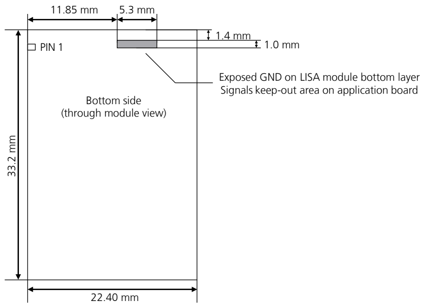
Figure 53: Signals keep-out area on the top layer of the application board, below LISA-U1 series modules
