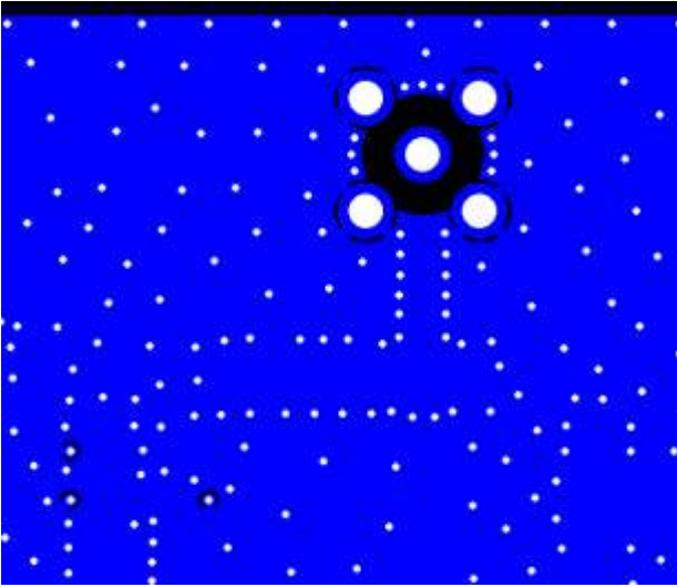
Figure 49: Layer 2 (inner layer) of u-blox approved interface board for LISA-U1 series modules
