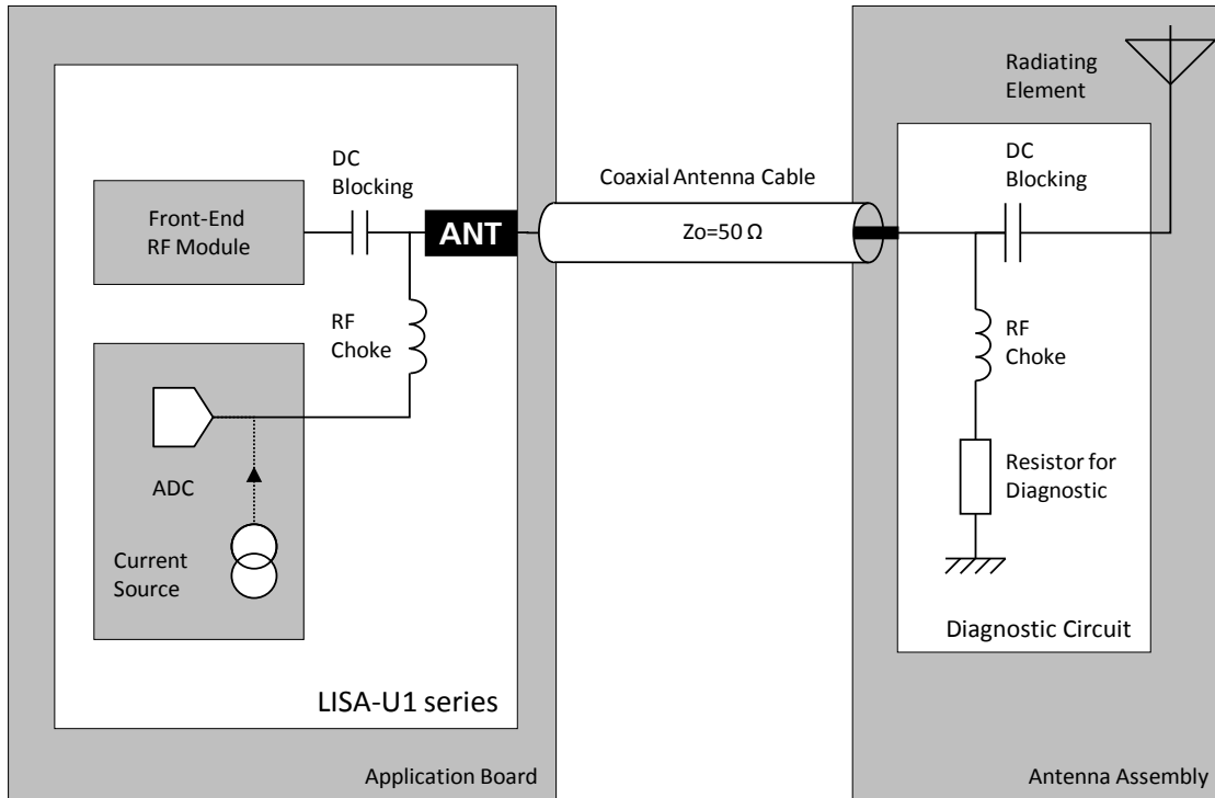
Figure 58: Antenna detection circuit and antenna with diagnostic resistor
