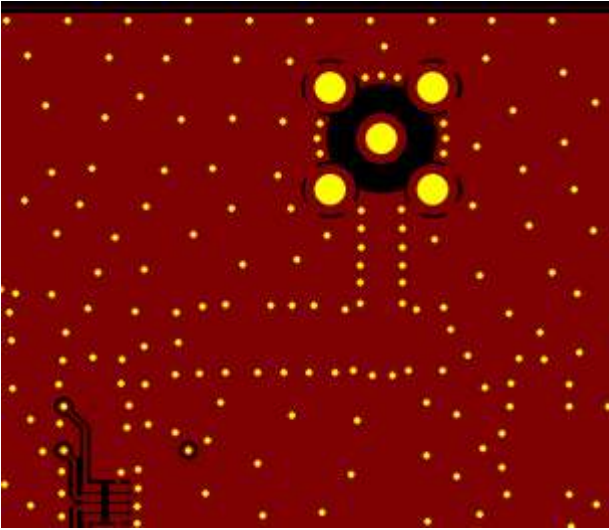
Figure 51: Layer 4 (bottom layer) of u-blox approved interface board for LISA-U1 series modules
