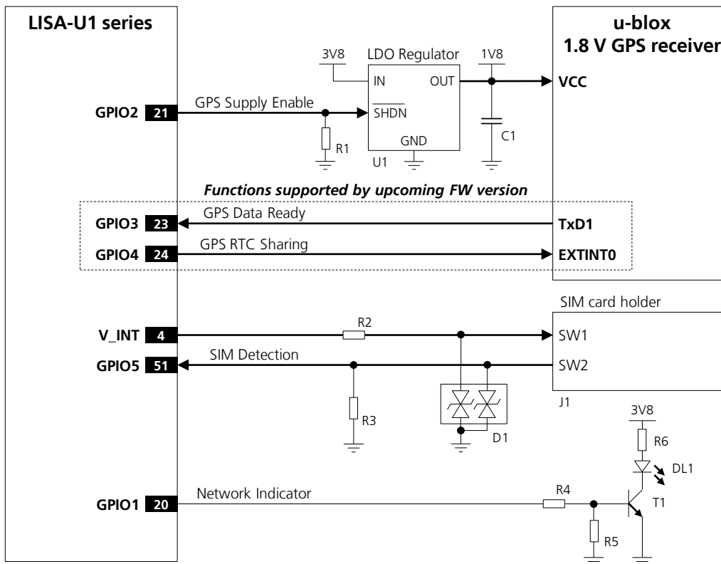
Figure 43: GPIO application circuit
