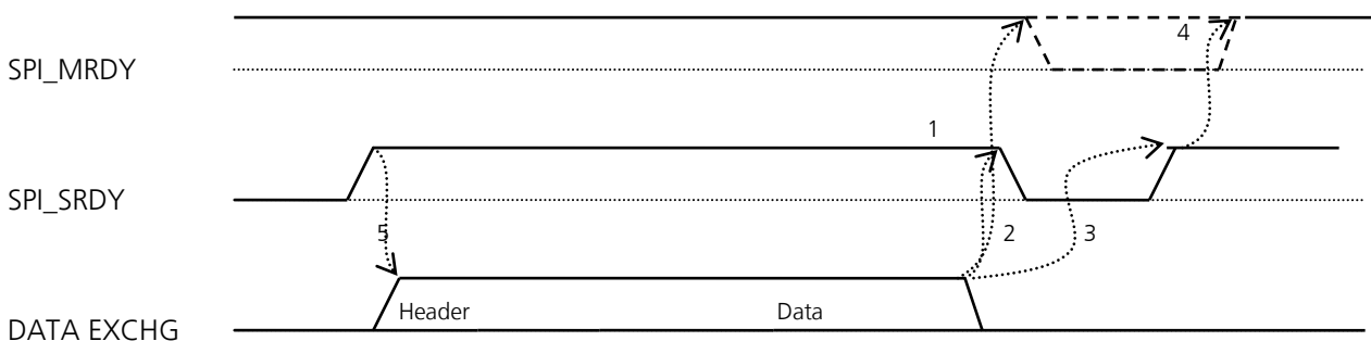
Figure 34: Data transfer terminated and then restarted by LISA-U1 series module (slave)
